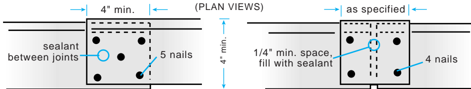
LAP JOINT DETAIL (preferred)
