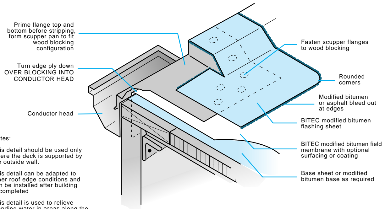
Cut-away view thru-scupper
